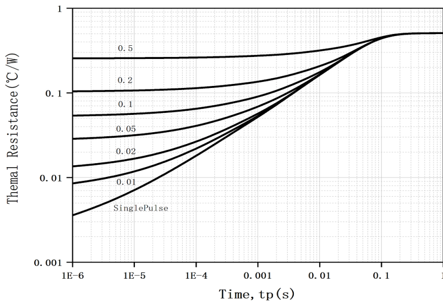
Figure 19. Transient Junction to Case Thermal Impedance
