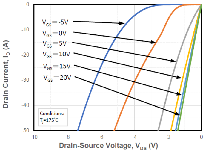
Figure 9. Reverse Output Characteristics at T_j = 175^\circ\text{C}
