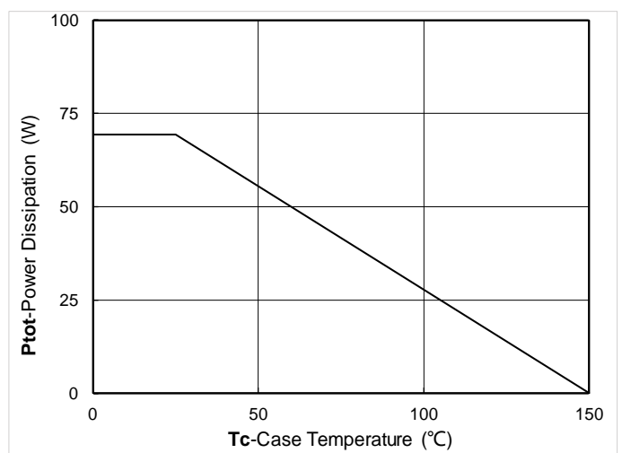
Figure 12. Power dissipation
